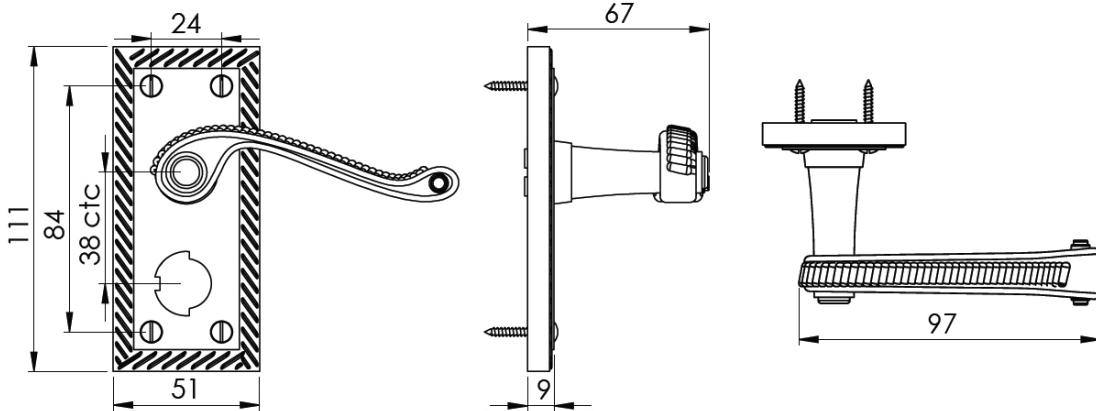
OUTSIDE VIEW With slotted release. Used to open door in emergency.
