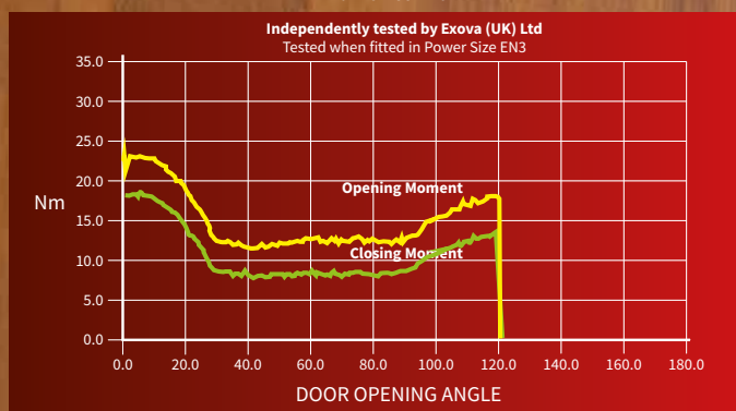
Power curve
